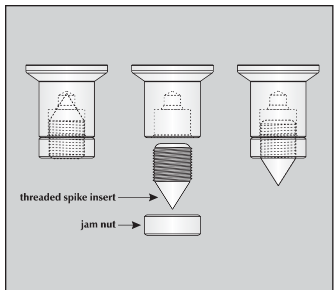
Figure 5. The ETC™ Spike.
