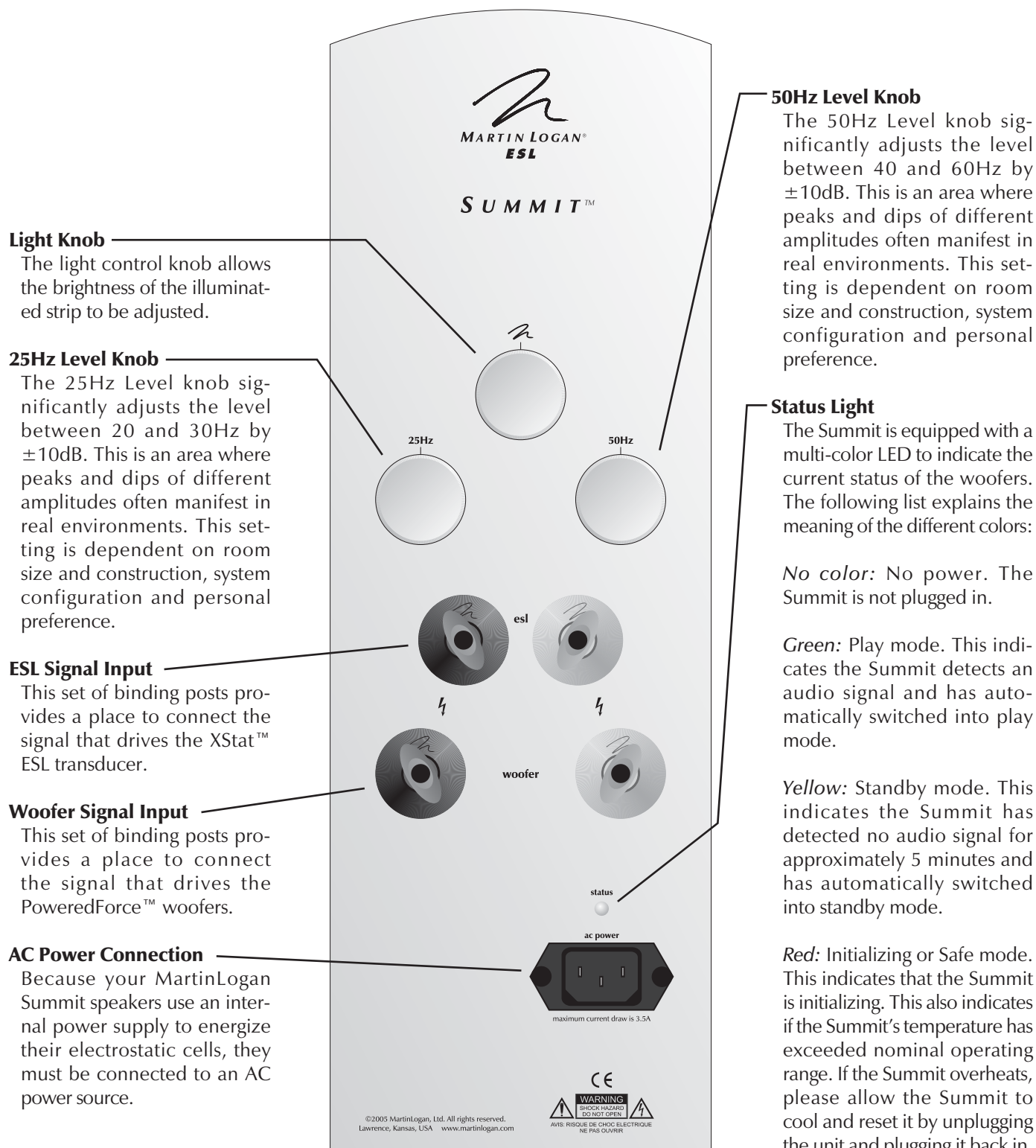
Figure 1. Summit Controls and Connections
